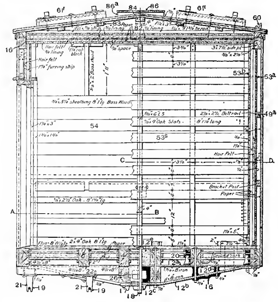
Fig. 281. Transverse Sections.
